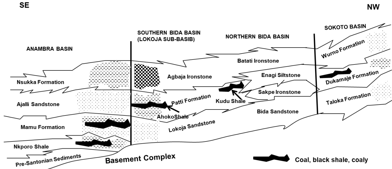
Fig. 2. Stratigraphy of Campanian-Maastrichtian formations in the Bida Basin correlated to the Anambra Basin and the Sokoto Basin (after Obaje, 2009).
